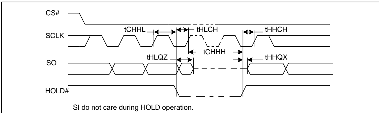
Figure28. Hold Timing
