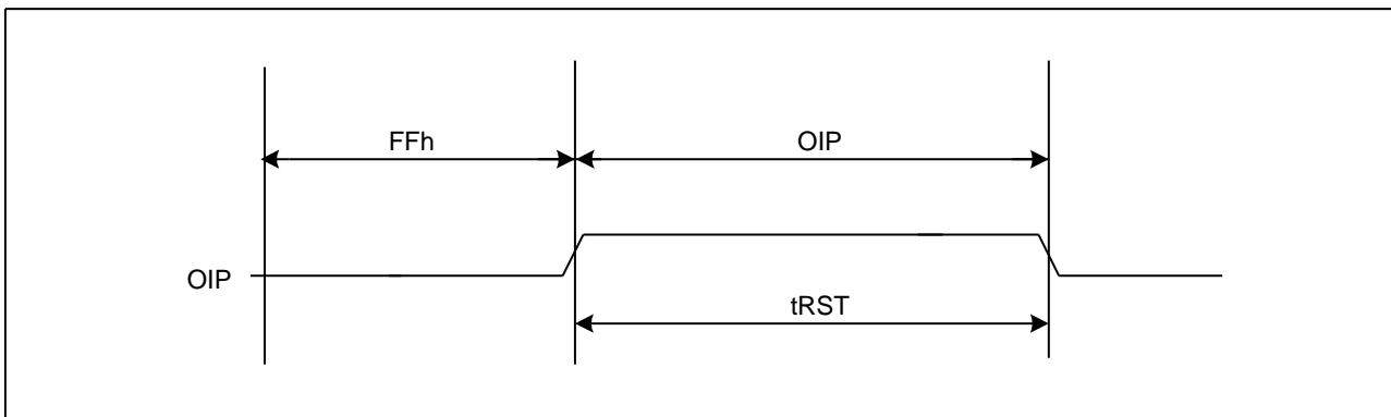
Figure29. Reset Timing
