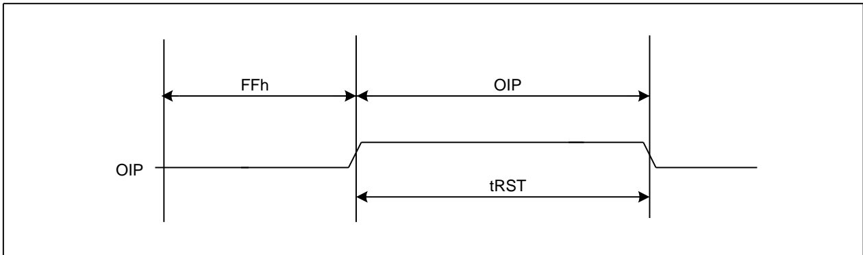
Figure28. Reset Timing
