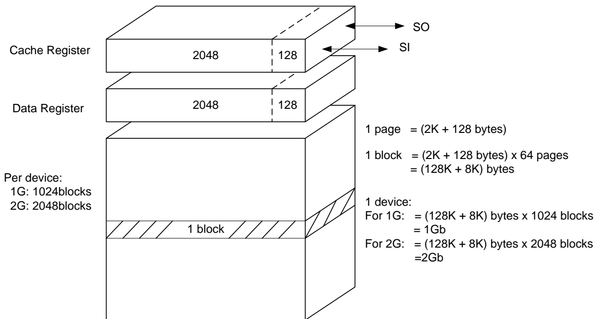
Figure1. Array Organization
