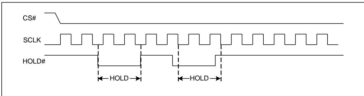
Figure3. Hold Condition
