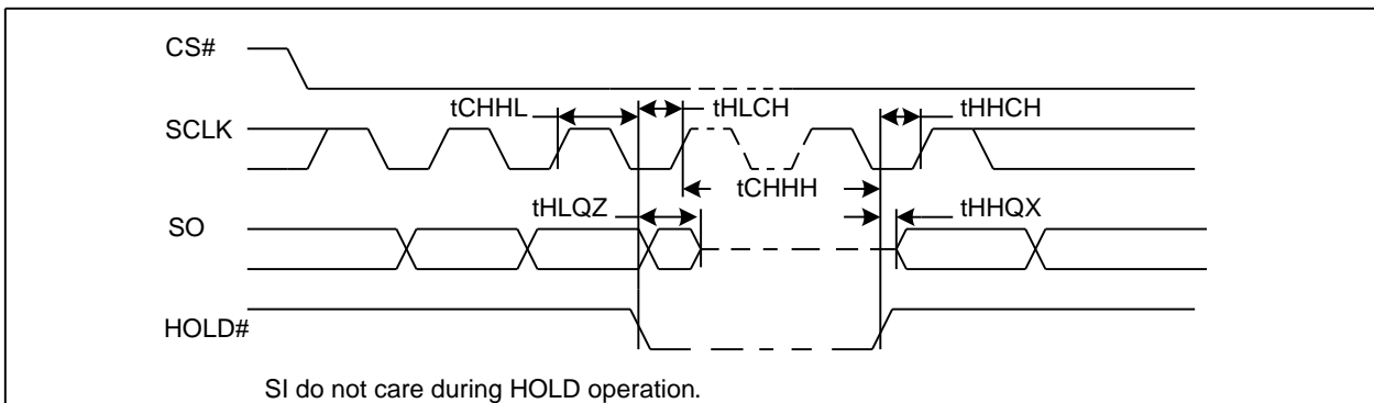
Figure27. Hold Timing
