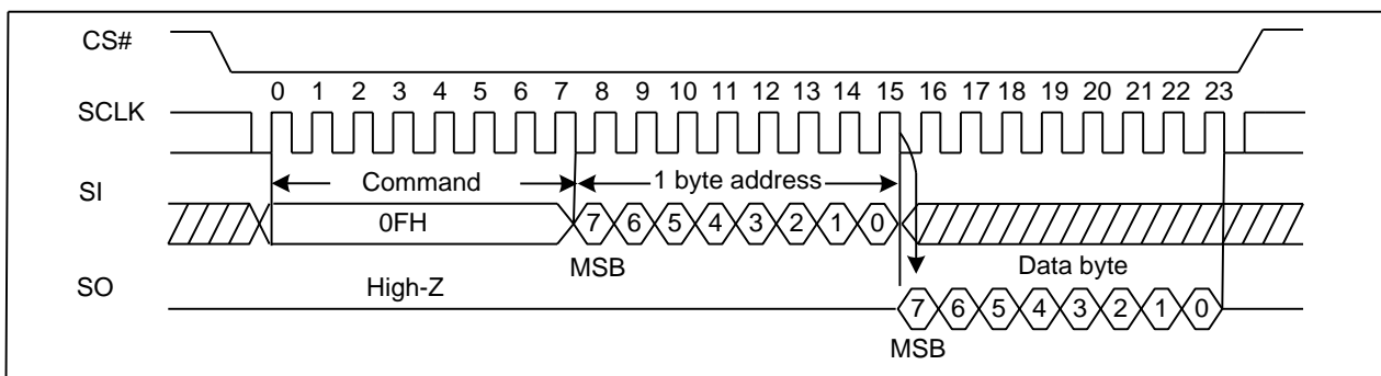
Figure6. Get Features Sequence Diagram
