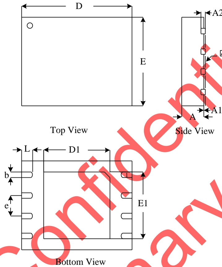
Figure30. WSON8 (8*6mm)
